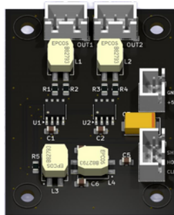
Étude du PCB Splitter AES/EBU 1 in / 2 out
